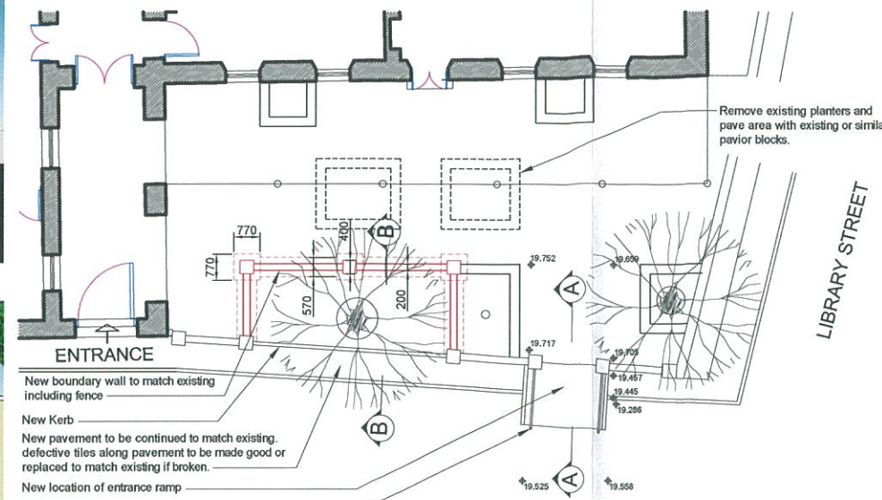
PROPOSED PLAN
